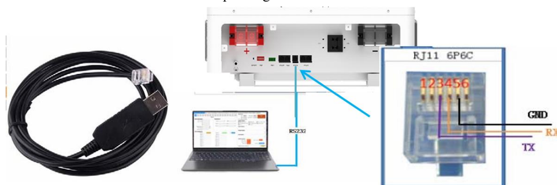
Figure 7 RS232 Serial port communication device
